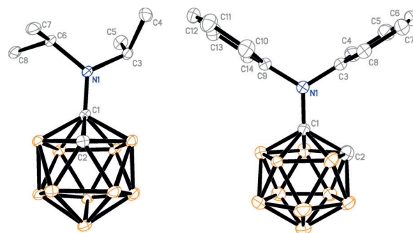
Figure 1. Molecular structures of 3e (left) and 3o (right). Selected bond distances [Å] and angles [°]. For 3e : C(1)–N(1) 1.369(2) Å, C(1)–C(2) 1.890(2) Å, N(1)–C(3) 1.481(2) Å, N(1)–C(6) 1.486(2) Å, C(1)–N(1)–C(3) 119.2(1)°, C(1)–N(1)–C(6) 124.5(2)°, C(3)–N(1)–C(6) 116.1(1)°; for 3o : C(1)–N(1) 1.402(3) Å, C(1)–C(2) 1.698(4) Å, N(1)–C(3) 1.441(3) Å, N(1)–C(9) 1.440(3) Å, C(1)–N(1)–C(3) 119.6(2)°, C(1)–N(1)–C(9) 122.5(2)°, C(3)–N(1)–C(9) 116.6(2)°.
